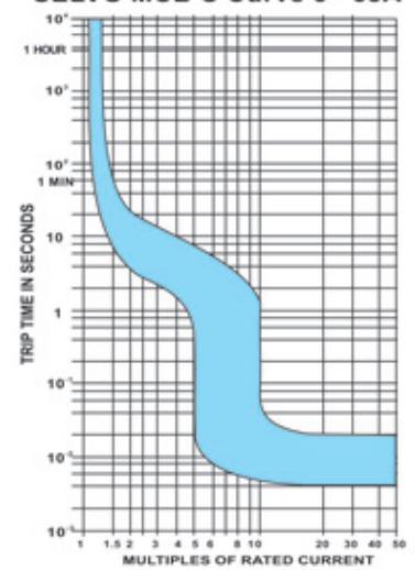
SELVO MCB C Curve 6 - 63A
