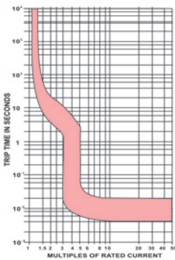
SELVO MCB B Curve 6 - 63A
